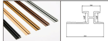
Model: 5503 Name: 5mm open I-bar Color: Matte Black, Matte Gold, Matte Prestige Gold, Rose Gold, Matte Ink Grey (from left to right)
