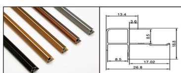
Model:8510 Name:8mm square external corner line Color:matte black,matte gold,matte prestige gold,rose gold,matte Ink grey(from left to right)
