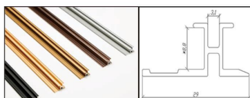
Model: 8503 Name: 8mm open I-bar Color: Matte Black, Matte Gold, Matte Prestige Gold, Rose Gold, Matte Ink Grey (from left to right)
