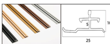
Model:8511 Name:8mm earth line Color:matte black,matte gold,matte prestige gold,rose gold,matte Ink grey(from left to right)
