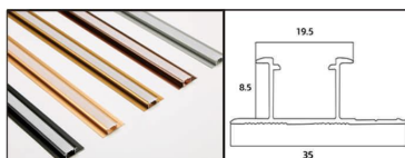
Model:8507 Name:8mm LED strip with I-bar Color:matte black,matte gold,matte prestige gold,rose gold,matte Ink grey(from left to right)
