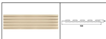
Name: 159 Small Great Wall Grille Size:159mm*9mm
