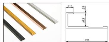
Model: 8501 Name: 8mm trimming line Color: Matte Black, Matte Gold, Rose Gold, Matte Ink Grey (from left to right)
