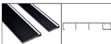
Model:8520 Name:8mm front illuminated skirting(upper)
