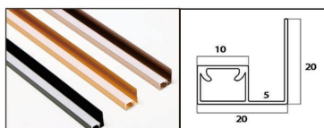
Model: 5516 Name: 5mm Vertical Light Strip Line Color: Matte Black, Matte Gold, Rose Gold (from left to right)
