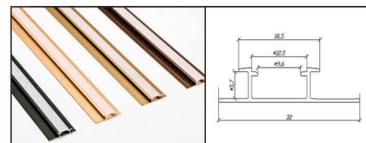
Model: 5507 Name: 5mm LED strip line Color: Matte Black, Matte Gold, Matte Prestige Gold, Rose Gold (from left to right)
