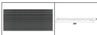
Name: 200 Triangle Grille Size:200mm*14mm
