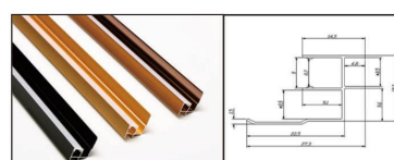
Model:8512 Name:8mm staggered light strip line Color:Matte Black,Matte Gold,Rose Gold(from left to right)
