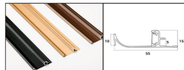
Model: 5513 Name: 5mm bottom luminous loght strip skirting Color: Matte Black, Matte Gold, Rose Gold (from left to right)
