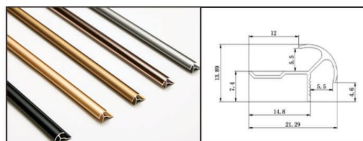
Model: 5508 Name: 5mm arc external line Color: Matte Black, Matte Gold, Matte Prestige Gold, Matte Ink Grey (from left to right)
