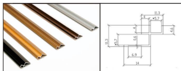
Model: 5505 Name: 5mm inner corner line Color: Matte Black, Matte Gold, Matte Prestige Gold, Rose Gold, Matte Ink Grey (from left to right)
