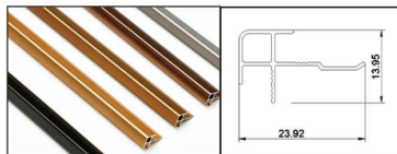
Model: 5510 Name: 5mm square external line Color: Matte Black, Matte Gold, Matte Prestige Gold, Rose Gold, Matte Ink Grey (from left to right)
