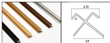
Model: 5506 Name: 5mm outer corner line Color: Matte Black, Matte Gold, Matte Prestige Gold, Rose Gold, Matte Ink Grey (from left to right)
